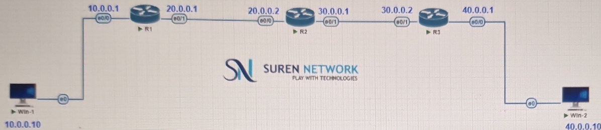
QEMU (Win-2)
